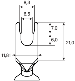
Multi-Spade Dimensions (mm)
