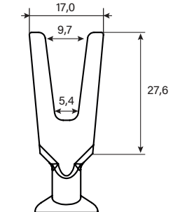
V-Spade Dimensions (mm)
