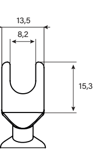
U-Spade Dimensions (mm)
